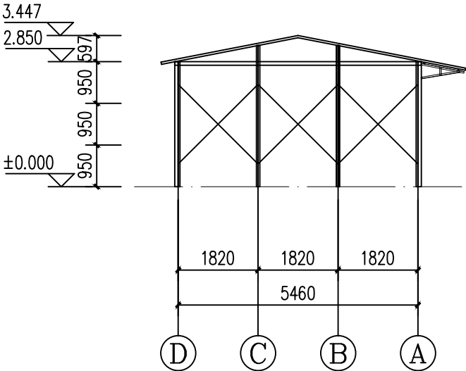
1-axis elevation
